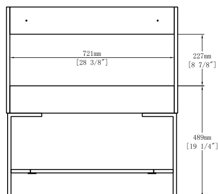
BACK VIEW
